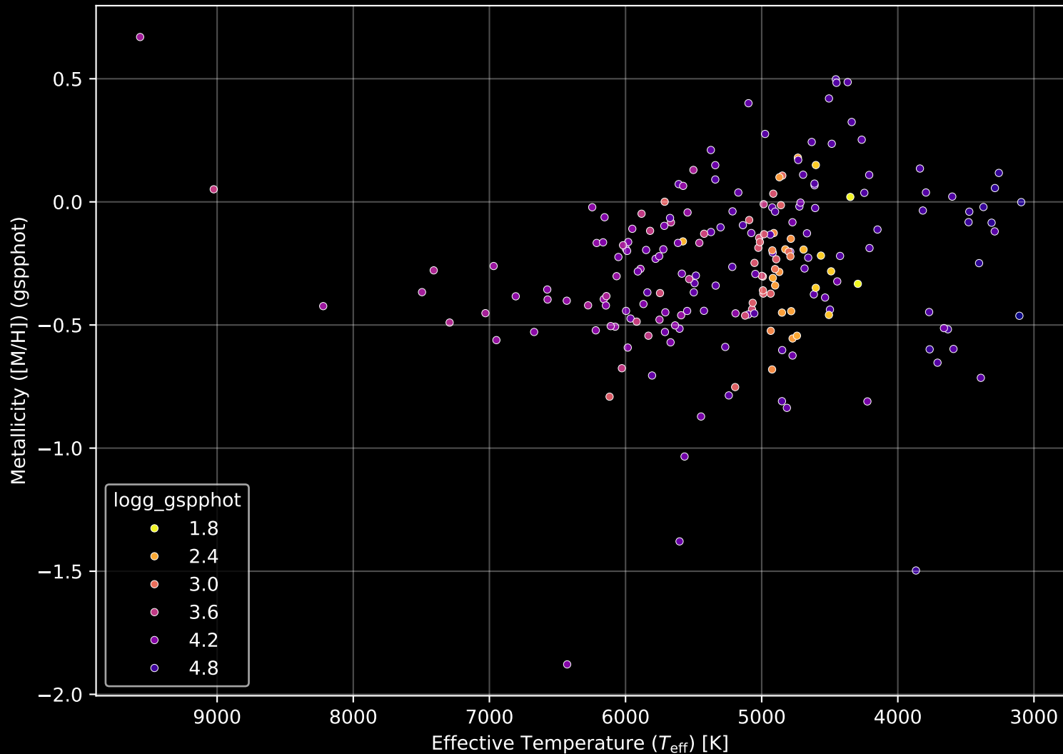
APOGEE DR17 Field: [K2_C5_208+29_btx] Stellar Population Parameters (n= 206)
