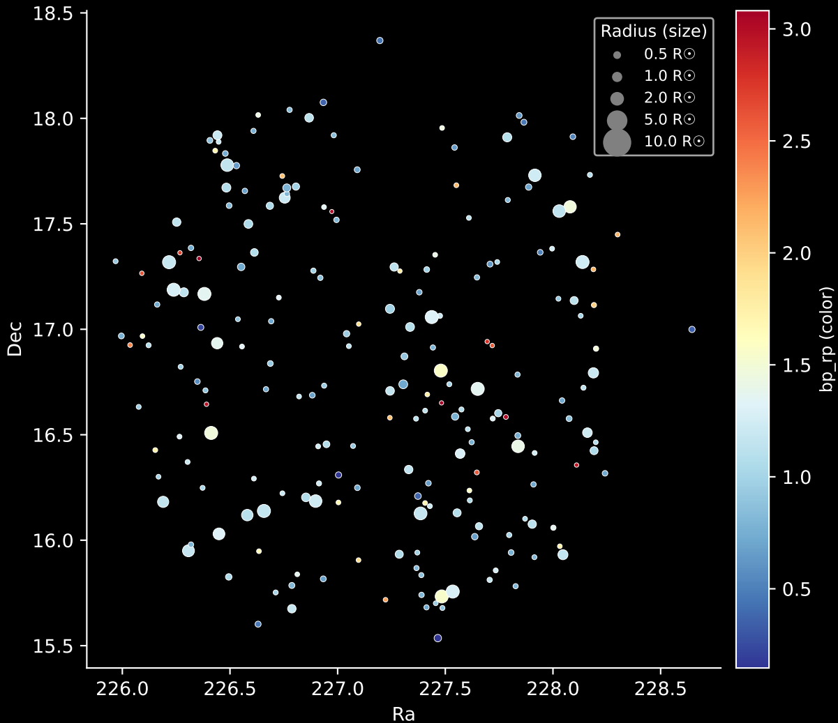
APOGEE DR17 Field: [K2_C5_208+29_btx] Stars: 206
