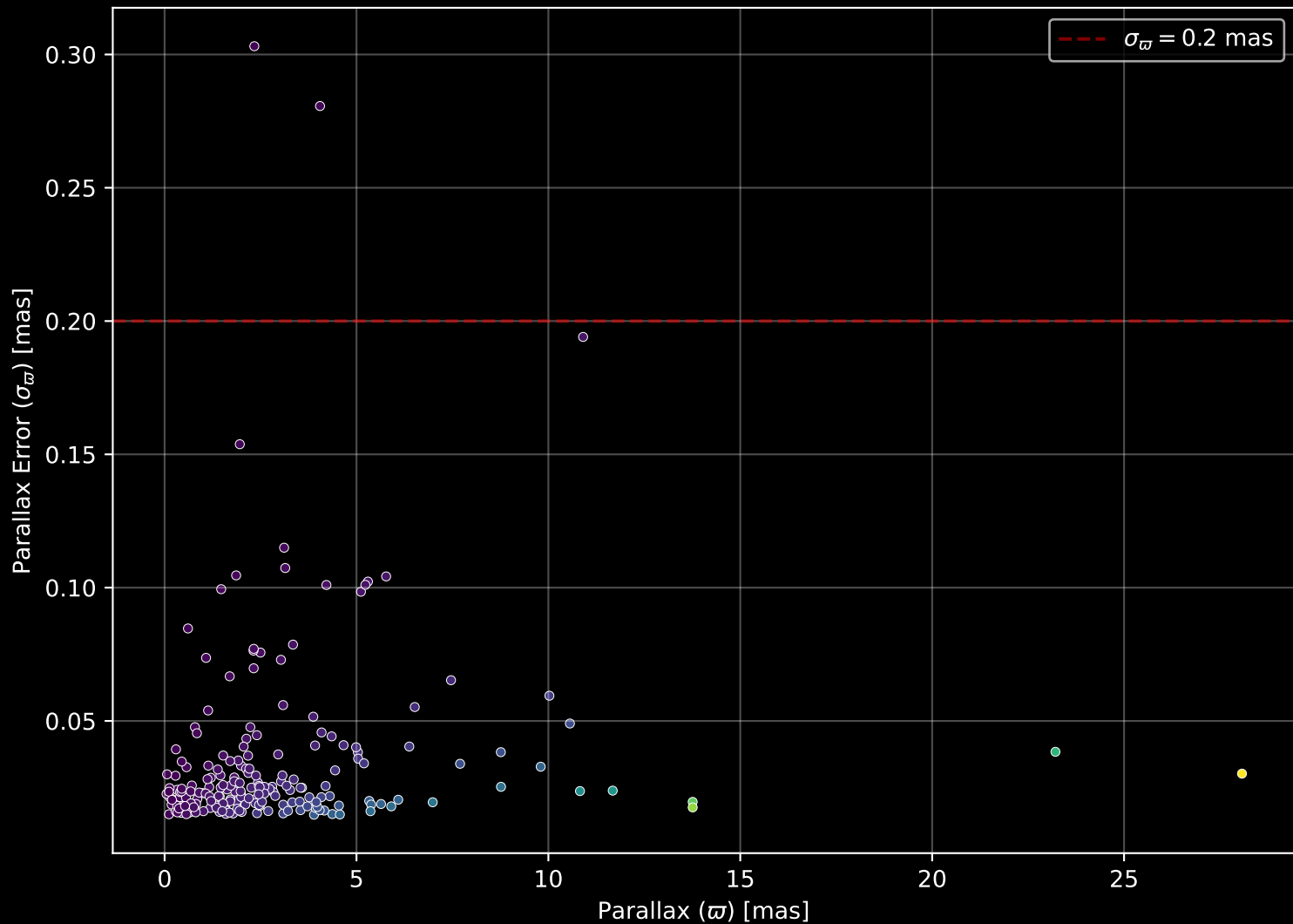
APOGEE DR17 Field: [K2_C5_208+29_btx] Parallax Quality (n= 206)
