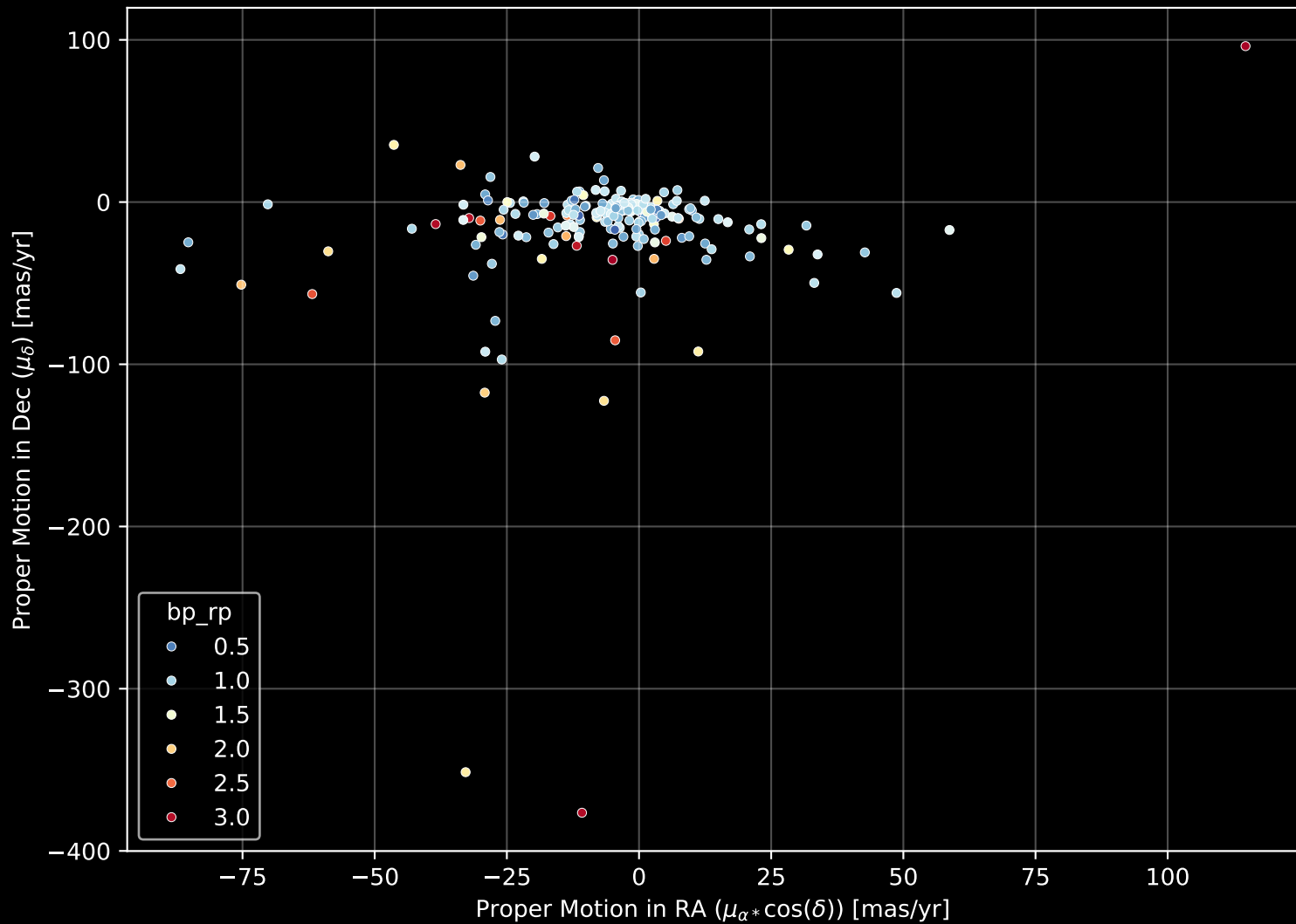
APOGEE DR17 Field: [K2_C5_208+29_btx] Proper Motion Diagram (n= 206)
