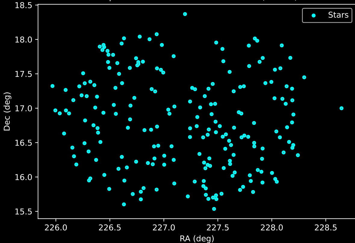
APOGEE DR17 Field: [K2_C5_208+29_btx] Proper Motion Vectors for Gaia Star Field (n= 206)
