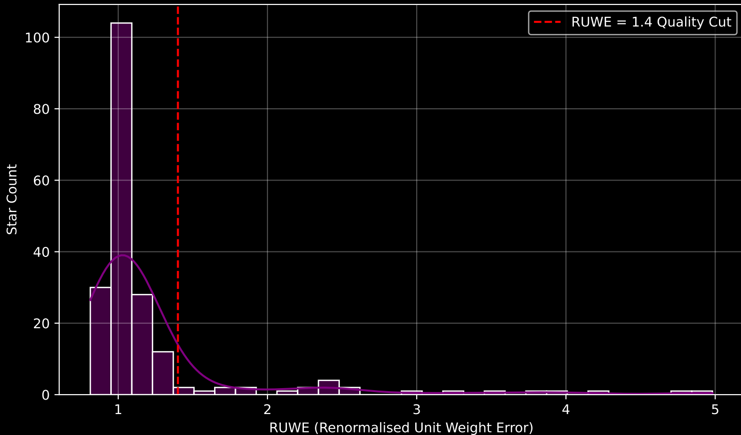
GAPOGEE DR17 Field [K2_C5_208+29_btx] RUWE Distribution (n= 198)
