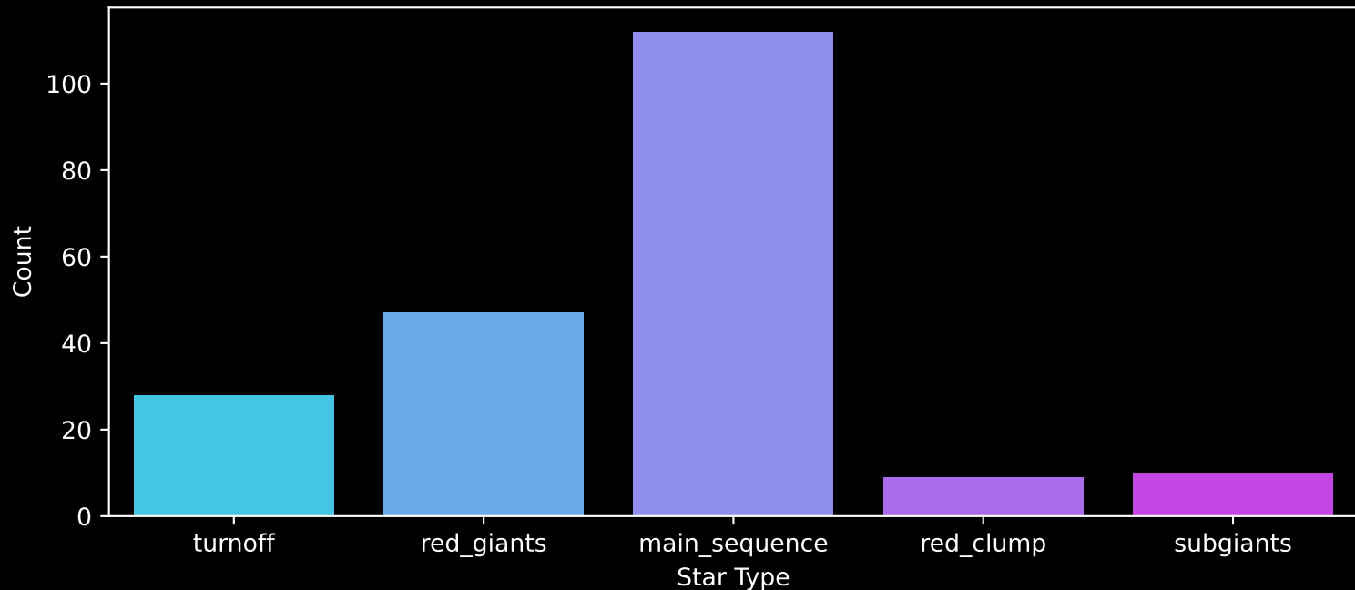
APOGEE DR17 Field: [K2_C5_208+29_btx] Count plot of Star Type
