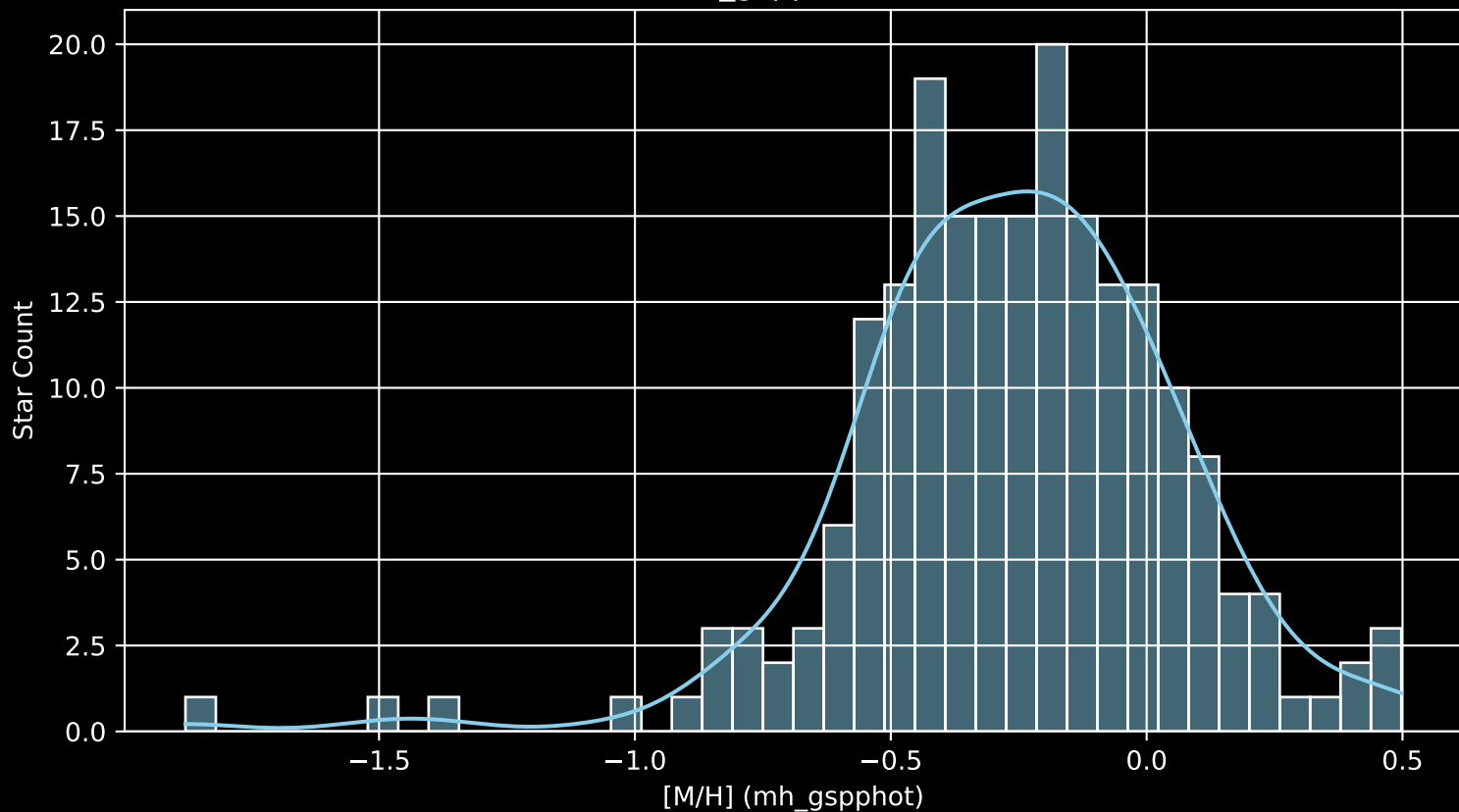
APOGEE DR17 Field: [K2_C5_208+29_btx [M/H] (mh_gspphot) (n= 205)
