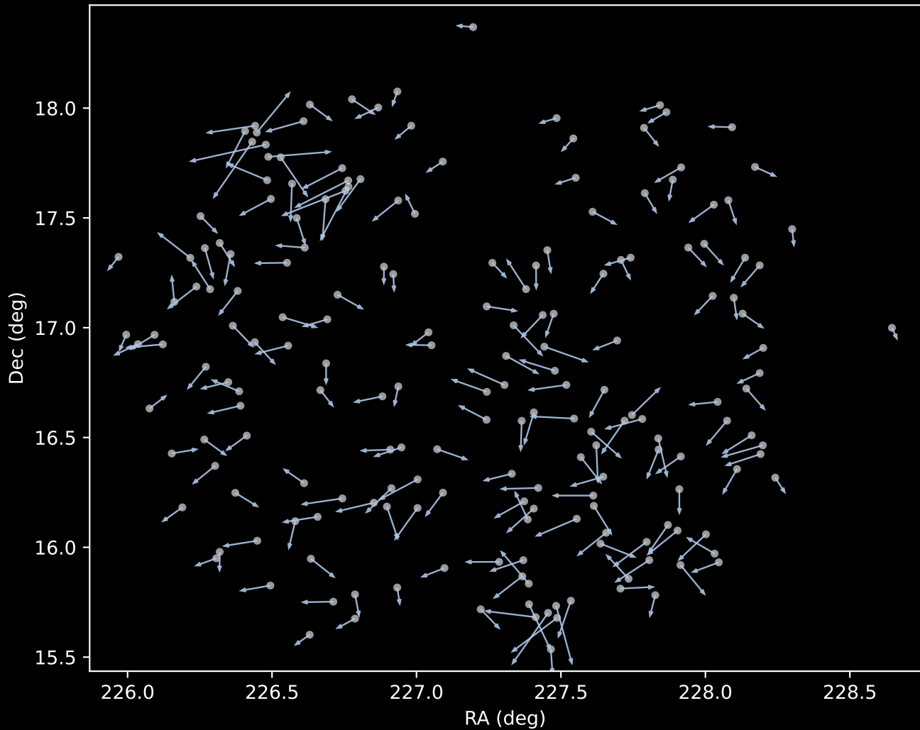
APOGEE DR17 Cluster 1 Proper Motion Vectors (n=192)
